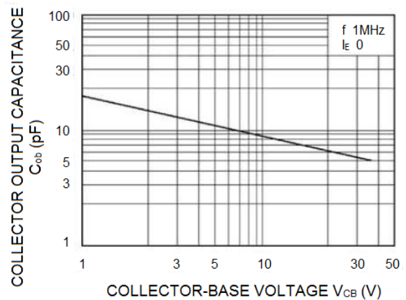
Figure 6. C_{ob} - V_{CB}
