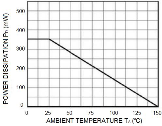
Figure 7. P_D - T_A
