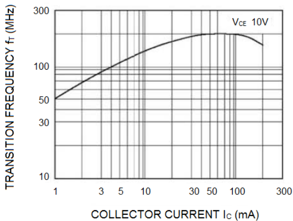
Figure 5. f_T - I_C
