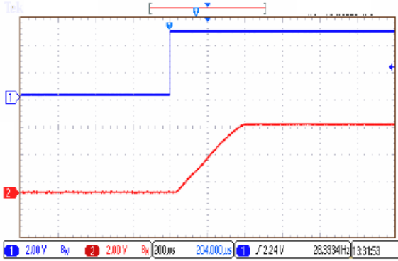
9. UVLO at Rising, CH1:VIN, CH2:VO
