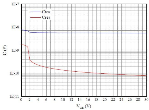
Fig.9 Capacitance characteristic
