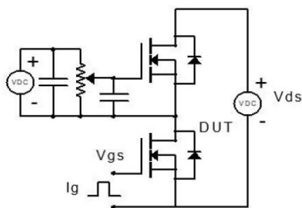
Fig 1. Gate Charge Test Circuit & Waveform
