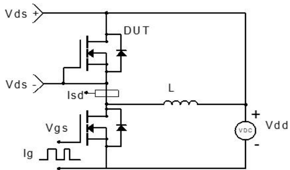
Fig 4. Diode Recovery Test Circuit & Waveform
