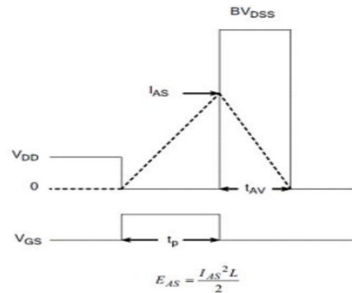
Fig 21. Unclamped Inductive Switching Waveform
