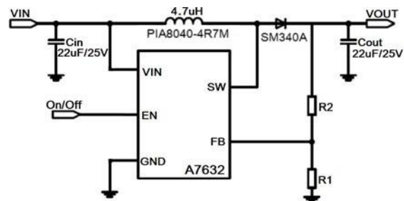
A7632 + PIA8040-4R7M + SM340A
