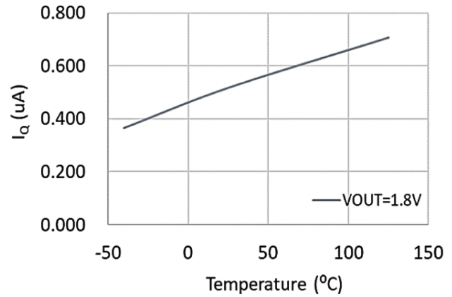
Fig 10. I_Q vs. Temperature
