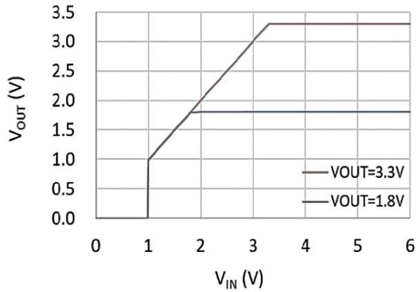
Fig 7. V_{OUT} vs. V_{IN}
