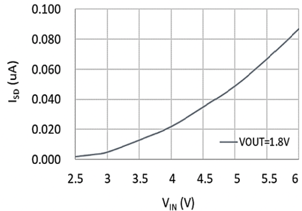
Fig 12. I_{SD} vs. V_{IN}
