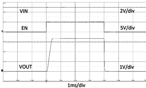
Fig 5. EN Enabled and Disabled
