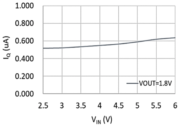
Fig 9. I_Q vs. V_{IN}
