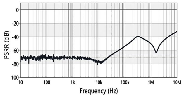
Fig 6. PSRR ( V_{IN} = 3.8V , V_{OUT} = 2.8V , I_{OUT} = 10mA )
