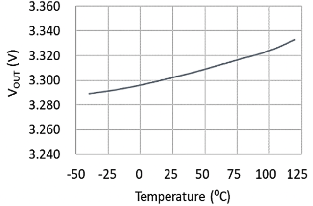
Fig 8. V_{OUT} vs. Temperature
