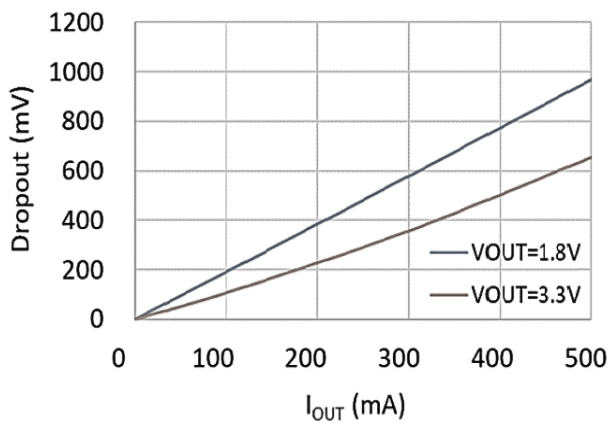
Fig 11. Dropout Voltage vs. I_{OUT}
