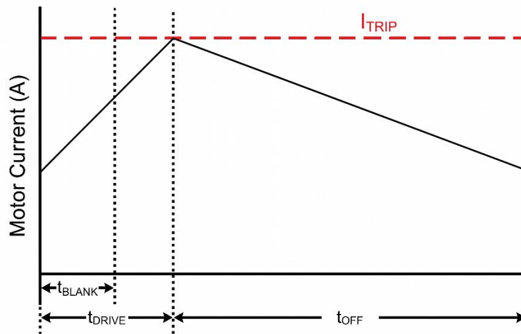
Fig 2. Current-Regulation Time Periods
