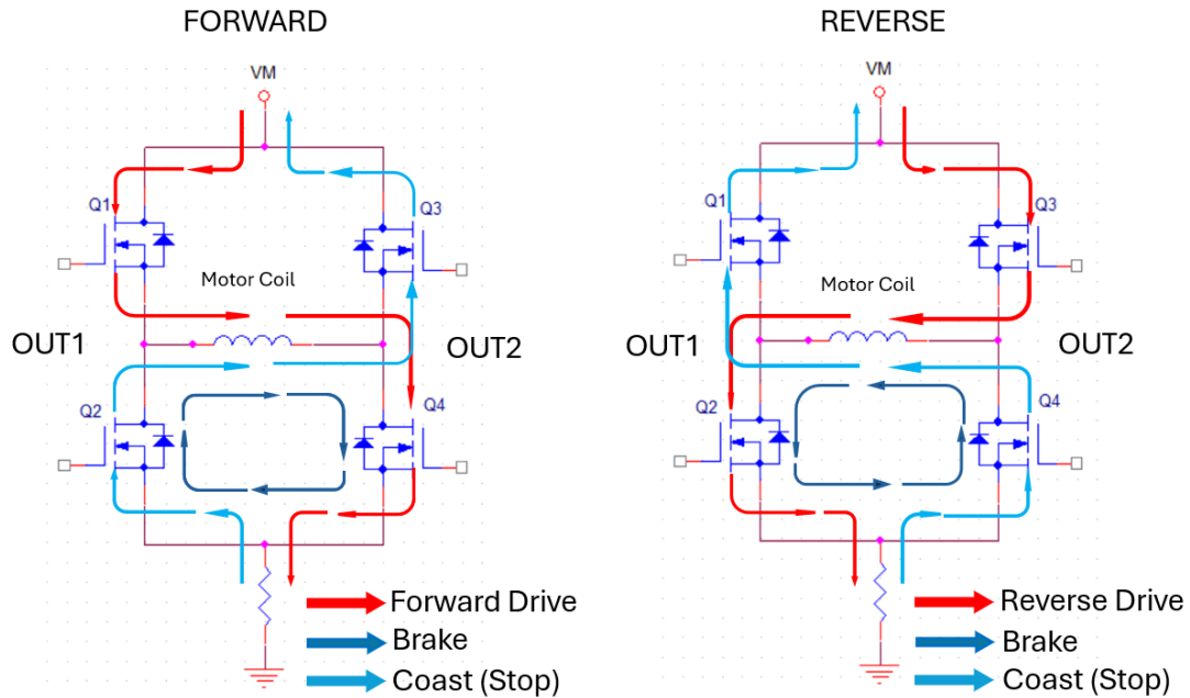
Fig1. H-Bridge Current Paths
