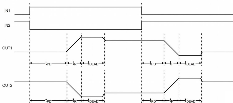
Fig 3. Propagation Delay Time
