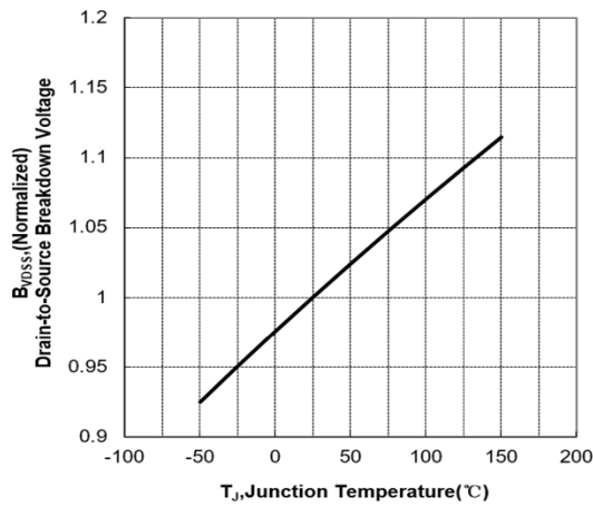
Fig 9. Typical Breakdown Voltage vs. Junction Temperature
