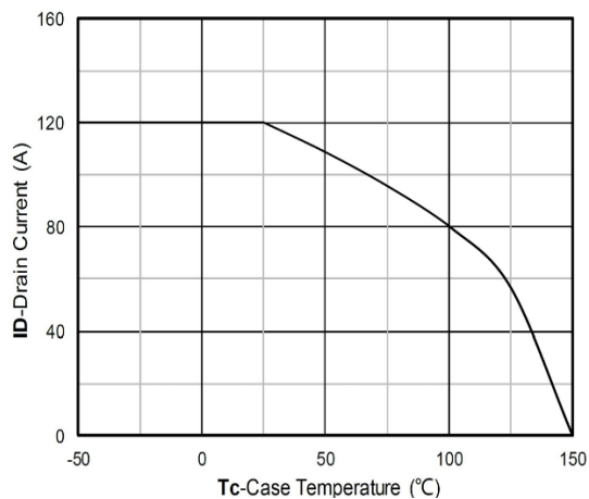
Fig 5. Current dissipation
