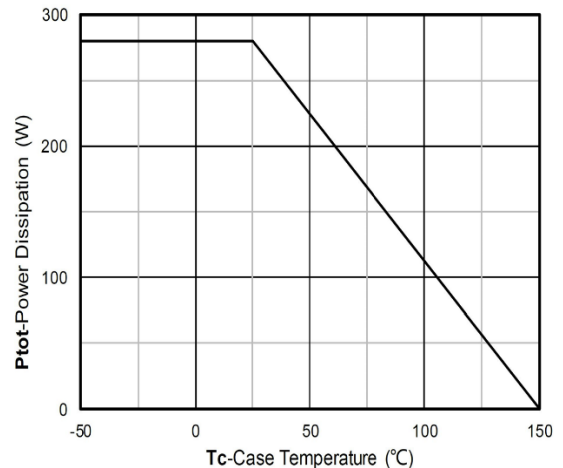
Fig 6. Power dissipation
