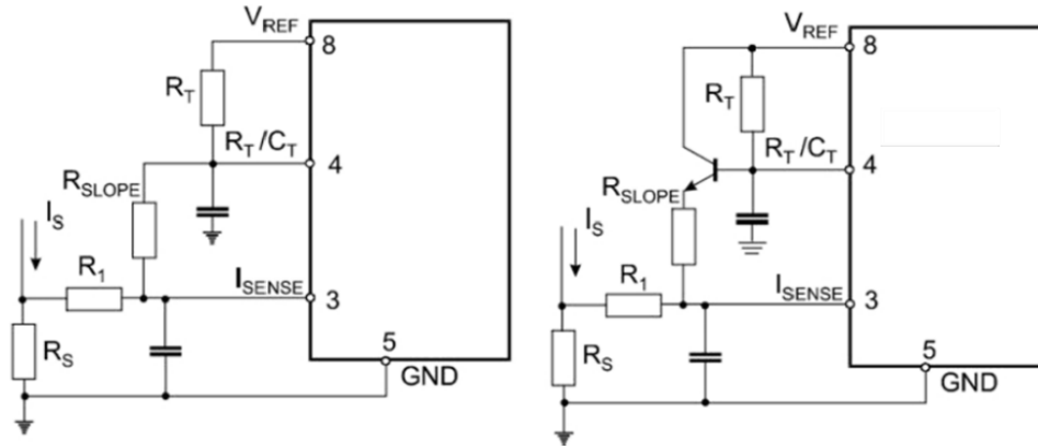
Fig 13. Slope Compensation Techniques
