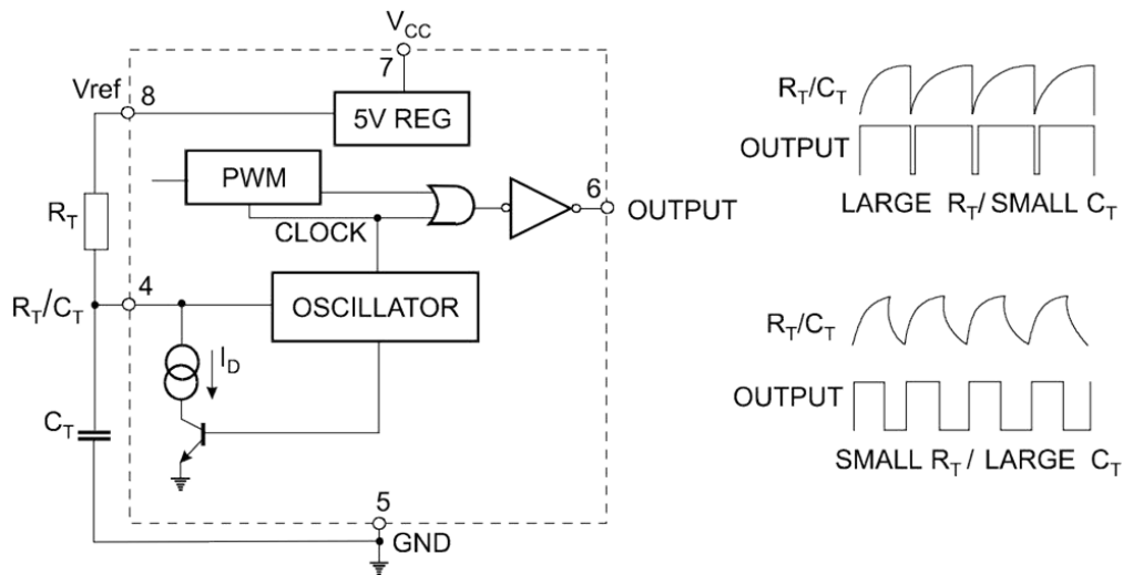
Fig 9. Oscillator and Output Waveforms
