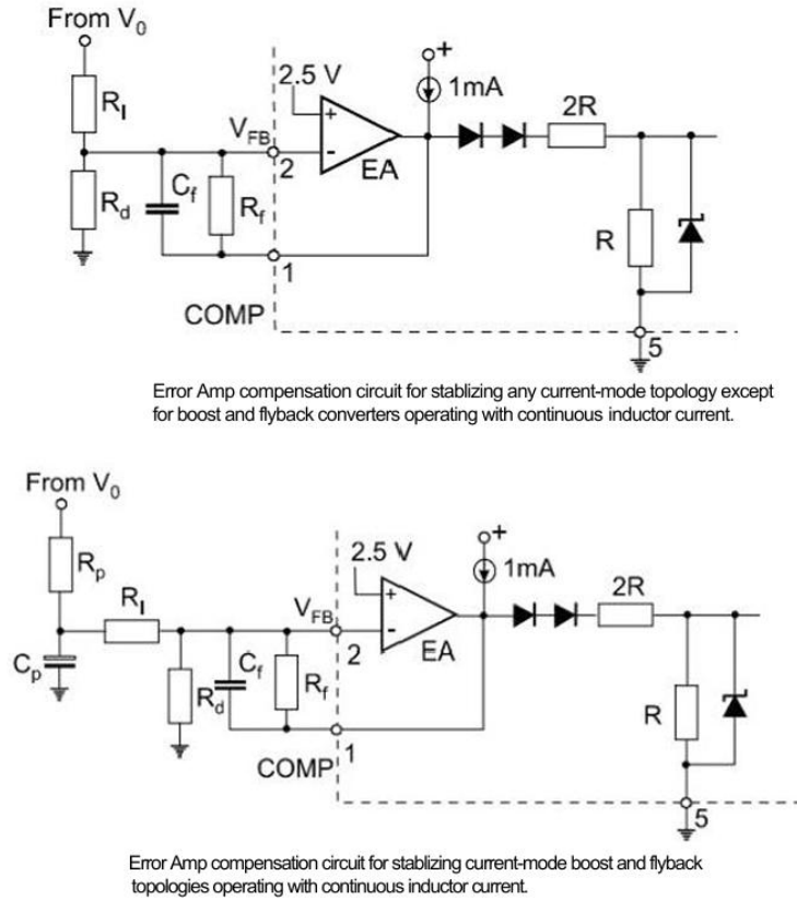
Fig 15. Error Amplifier Compensation
