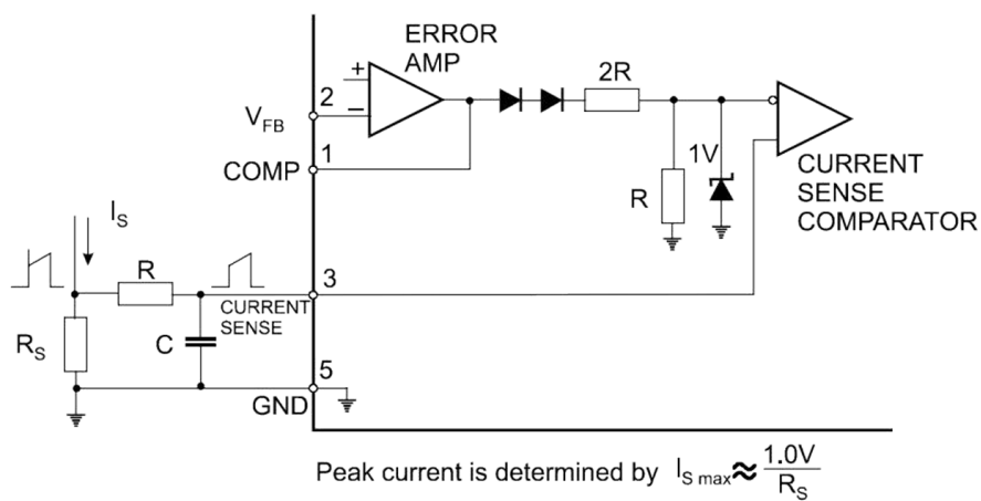
Fig 12. Current Sense Circuit
