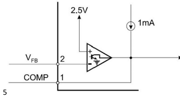
Fig 10. Error Amp Configuration
