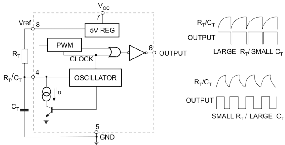
Fig 9. Oscillator and Output Waveforms
