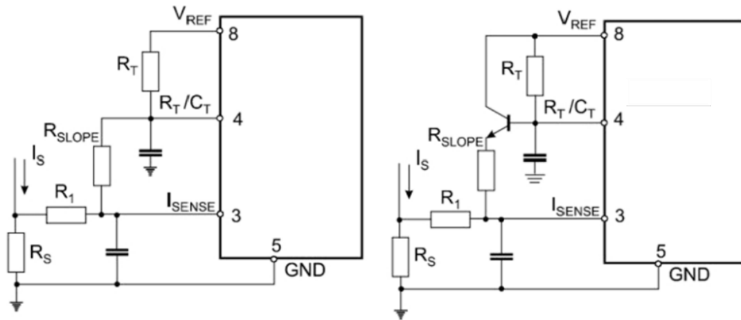
Fig 13. Slope Compensation Techniques
