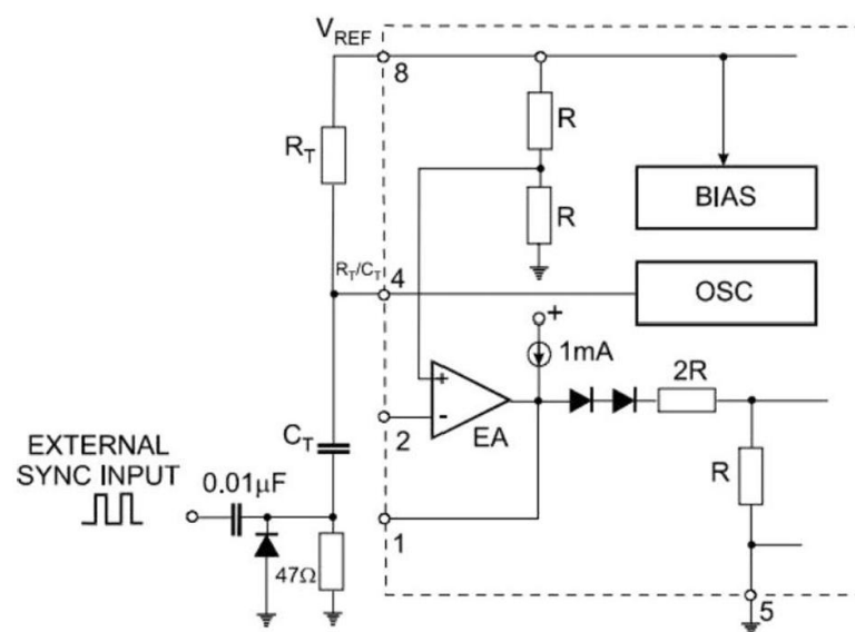
Fig 16. External Clock Synchronization
