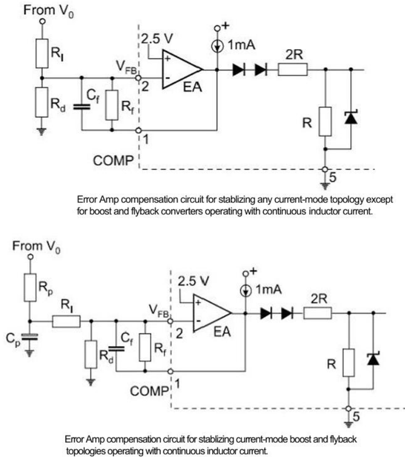
Fig 15. Error Amplifier Compensation
